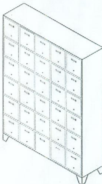
SS SHOE LOCKER CABINET
